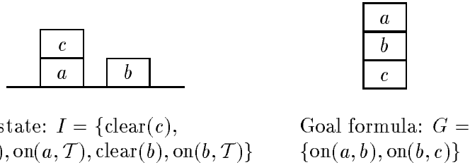
Figure 4: Sussman’s anomaly.
