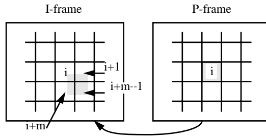
Figure 5.3: Macroblock Dependencies and Frame Interleaving. This figure shows a sample scenario of interleaving with m macroblocks per line. In the decompression of the i th P-frame macroblock with interleaving, the algorithms must make sure the I-frame stays “ahead” of the macroblocks that will depend on it. Thus, in the decompression of the i th macroblock in the P-frame, the macroblocks i , i+1 , i+m , and i+m+1 in the I-frame will be already decoded.
